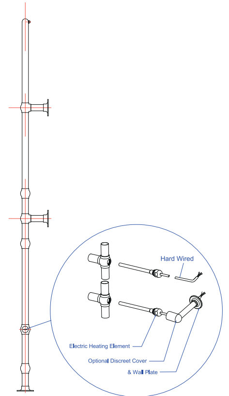
Heater Kit Assembly (UK)
