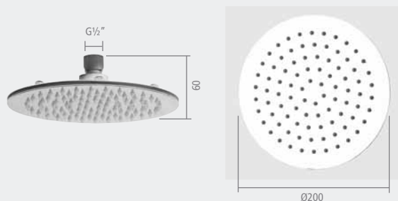
Round 200mm shower head (brass)
