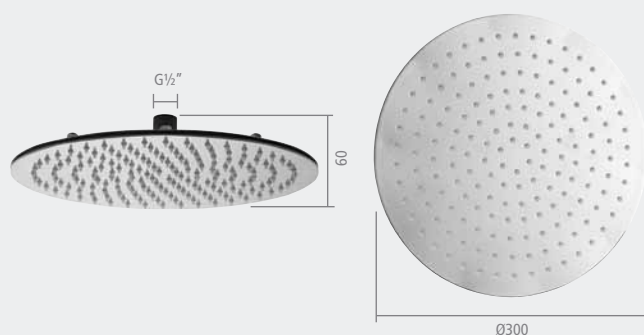
Round 300mm shower head (brass)
