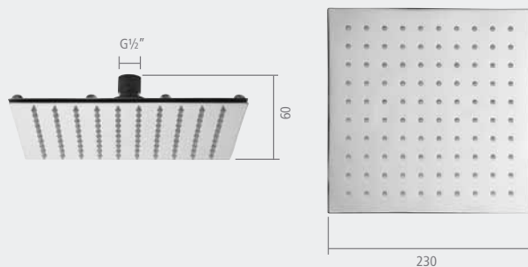
Square 230mm shower head (brass)
