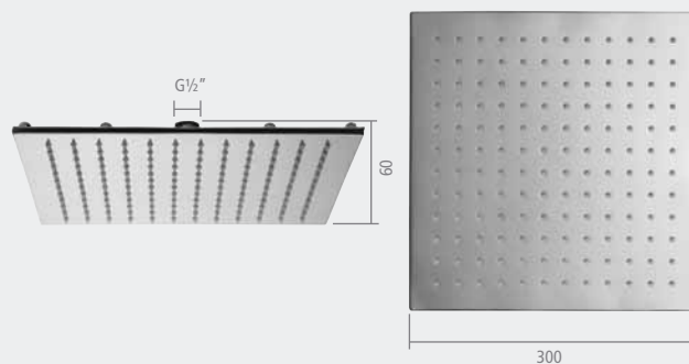
Square 300mm shower head (brass)
