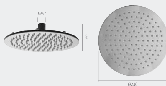
Round 230mm shower head (brass)
