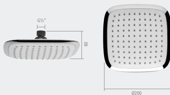
Square 200mm shower head
