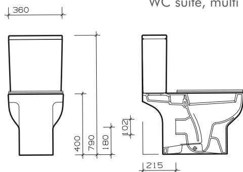
Quinta close coupled, washdown WC suite, multi outlet
