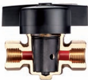
Valve with zero pressure loss for isolation
