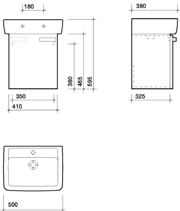
Galerie plan 500 x 380mm washbasin and furniture unit
