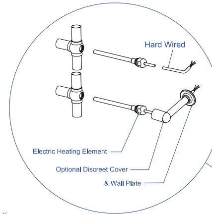
Heater Kit Assembly (UK)
