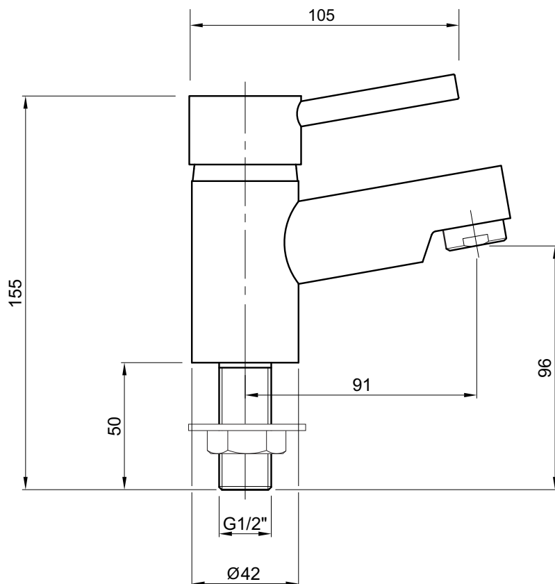
X60 Basin 1/2" Pillar Taps
