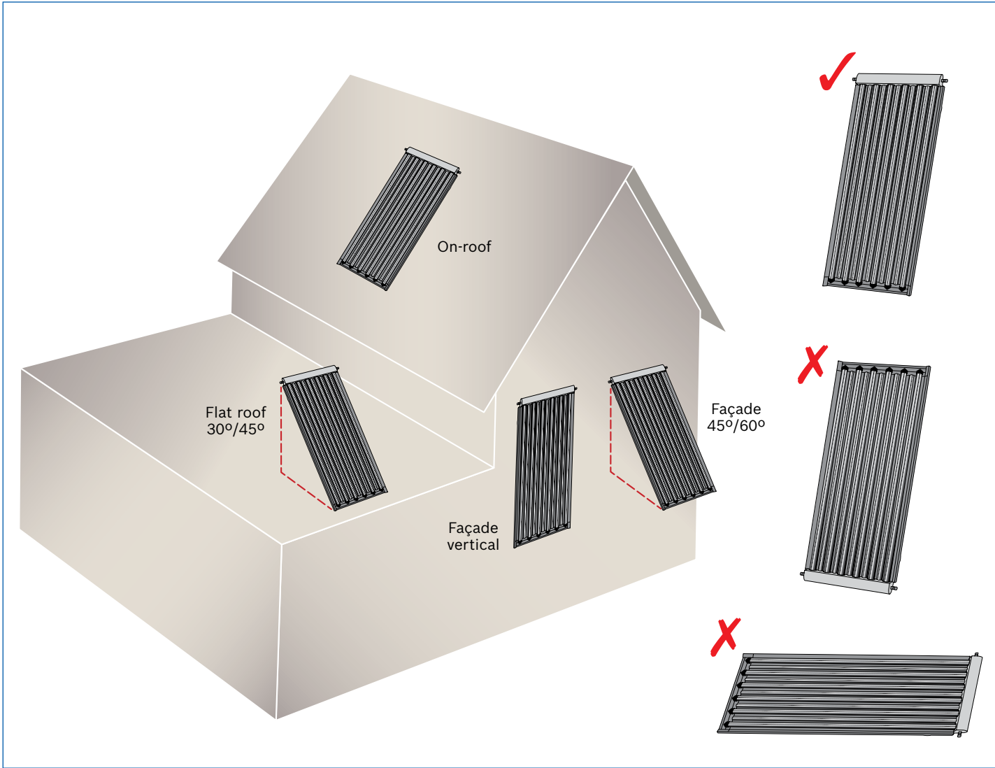
Collectors can only be installed vertically with the manifold at the top.
