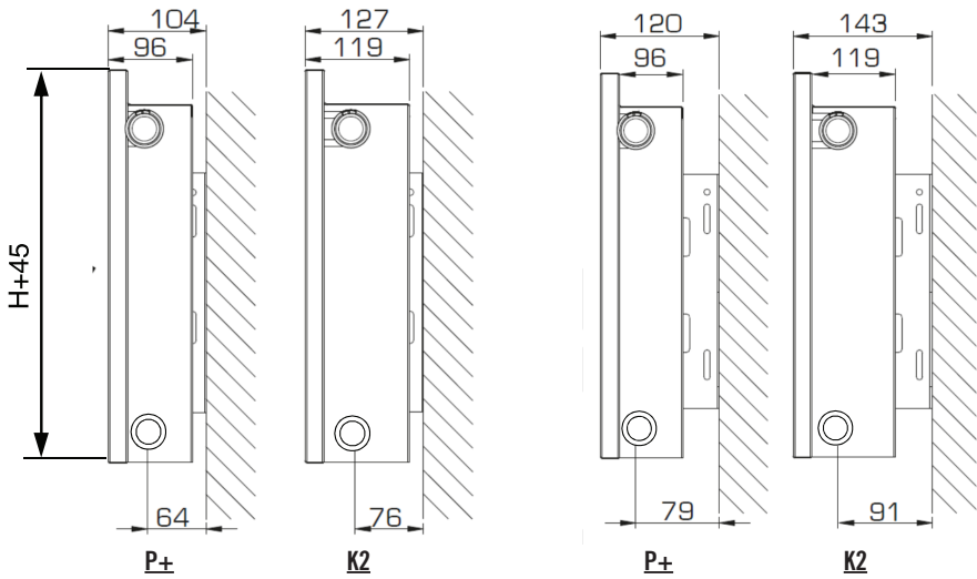
Mounting on short side of L-bracket
