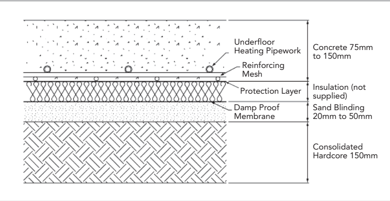
Mesh System (Concrete floor structure shown)
