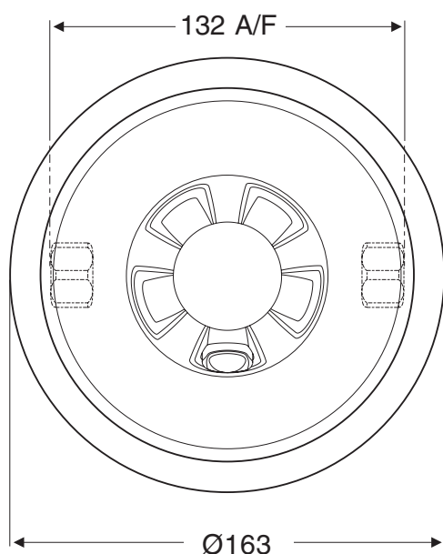
Mira CombiForce 415B
