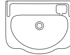
Reflections 60cm basin w605 x d470mm height – floor to rim 790
