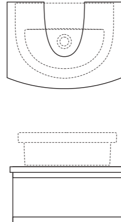
Washpoint Trend wall mounted 585mm vessel unit for 65 and 60cm pedestal basins and 45 and 50cm apron fronted basins w615 x d395 x h270mm
