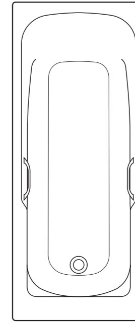
Admiral 167 x 69cm Idealform Plus+ bath 1675 x 690mm height – floor to rim 540-560mm
