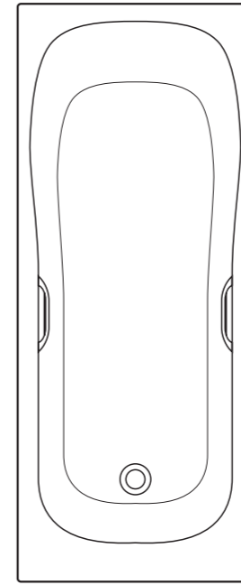
Marina 170 x 70cm Idealform Plus+ bath 1695 x 695mm height – floor to rim 540-560mm
