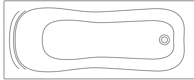
Caspian 170 x 70cm Idealcast bath 1695 x 695mm height – floor to rim 510-560mm
