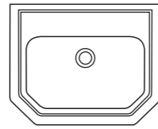
Plaza 58cm basin w580 x d465mm height – floor to rim 800
