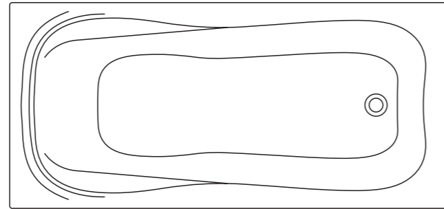
Caspian 170 x 80cm Idealcast bath 1695 x 795mm height – floor to rim 510-560mm
