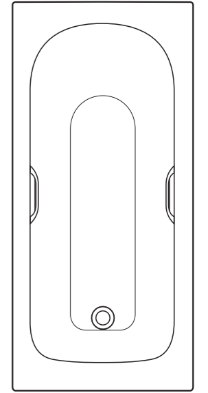
Harrow 150 150 x 70cm Idealform or Idealform Plus+ bath with optional grips, 1500 x 700mm height – floor to rim 540-560
