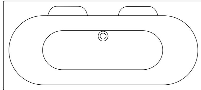
Linda 180 x 80cm Idealform bath 1795 x 795mm height – floor to rim 515-540mm
