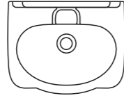
Reflections 45cm cloakroom basin 45cm handrinse basin w450 x d360mm height – floor to rim 805
