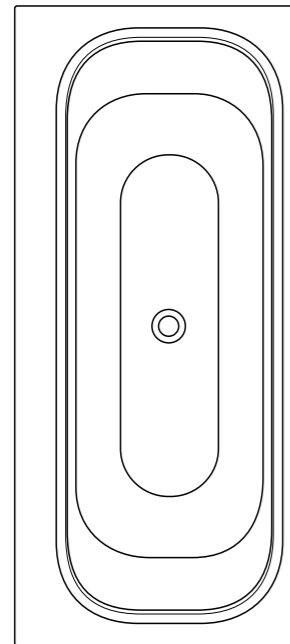
Jasper Morrison 170 x 75cm Idealform bath 1695 x 745mm height – floor to rim 595mm
