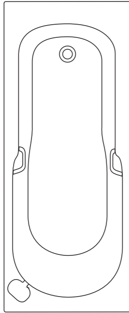
Studio 170 x 70cm Idealform bath 1695 x 695mm height – floor to rim 480-540mm
