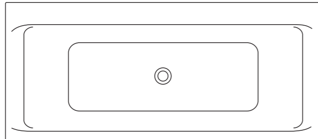
Washpoint 170 x 75cm Idealform Duo bath 1695 x 745mm height – floor to rim 555-595mm
