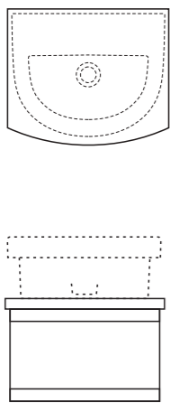
Washpoint Trend wall mounted 440mm vessel unit for 45cm apron fronted handrinse basin w470 x d395 x h270mm
