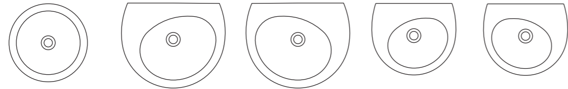
Edge 42cm vessel basin w420 x d420mm h185mm Drift 56cm basin right handed w560 x d460mm h815mm (floor to rim) Drift 56cm basin left handed w560 x d460mm h815mm (floor to rim) Drift 45cm handrinse basin right handed w450 x d385mm Drift 45cm handrinse basin left handed w450 x d385mm
