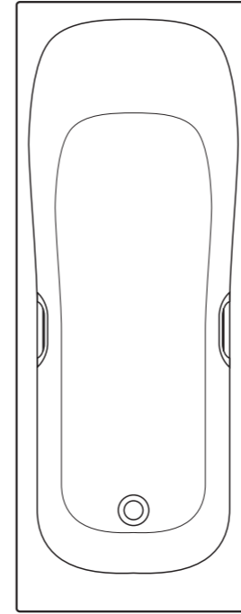
Marina 180 x 70cm Idealform Plus+ bath 1795 x 695mm height – floor to rim 540-560mm
