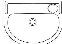
Revue 60cm basin w600 x d475mm height – floor to rim 800
