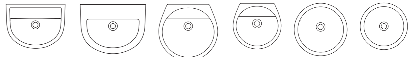
Washpoint 50cm under- countertop basin w500 x d380mm Washpoint 55cm apron fronted semi-countertop basin w555 x d420mm White round 50cm basin w500 x d485mm White round 40cm basin w400 x d390mm White round 45cm semi- countertop basin w450 x d450mm White round 40cm vessel basin w400 x d400mm
