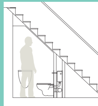
Staircase elevation
