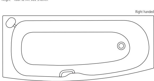
Studio 170 x 70cm Idealform spacemaker right handed bath 1695 x 695mm height – floor to rim 500-540mm
