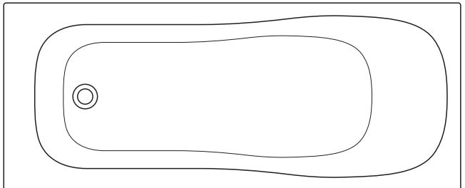
Create 170 x 70cm Idealform bath 1700 x 695mm height – floor to rim 540mm bath screen/over-bath enclosure height – 1500mm
