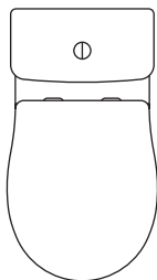
Square close coupled wc suite w360 x d500mm h790mm
