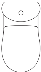
Drift close coupled wc suite w360 x d650mm h790mm
