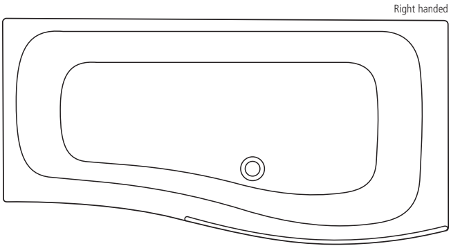
Create 170cm Idealcast shower bath right handed 1700 x 700mm (850mm at widest point) height – floor to rim 540mm bath screen/ over-bath enclosure height – 1500mm
