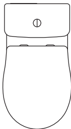
Edge close coupled wc suite w360 x d650mm h790mm
