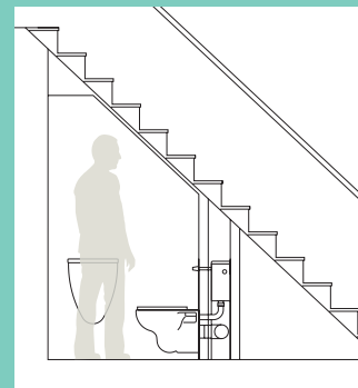
Staircase elevation
