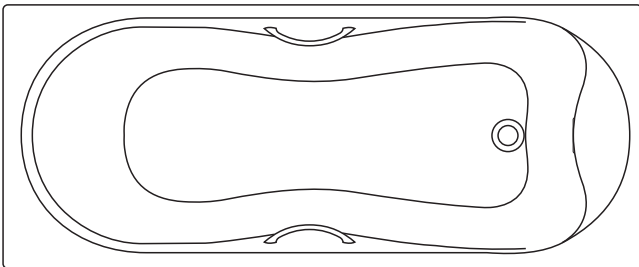
Purity 170 x 70cm Idealform bath 1700 x 700mm height – floor to rim 500-540mm
