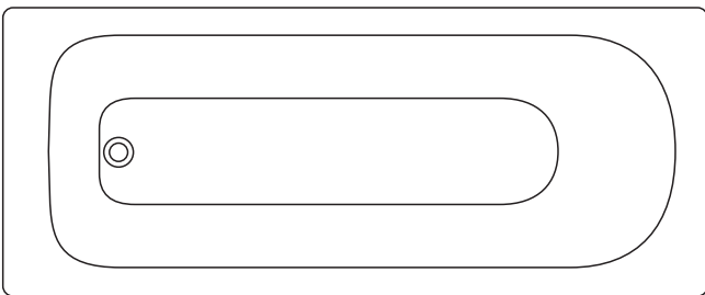
Harrow 170 170 x 70cm Idealform bath or Idealform Plus+ bath with optional grips, 1695 x 695mm height – floor to rim 545
