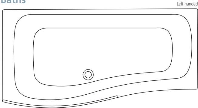
Create 170cm Idealcast shower bath left handed 1700 x 700mm (850mm at widest point) height – floor to rim 540mm bath screen/ over-bath enclosure height – 1500mm
