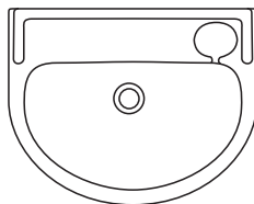
Revue 60cm basin w600 x d475mm height – floor to rim 800
