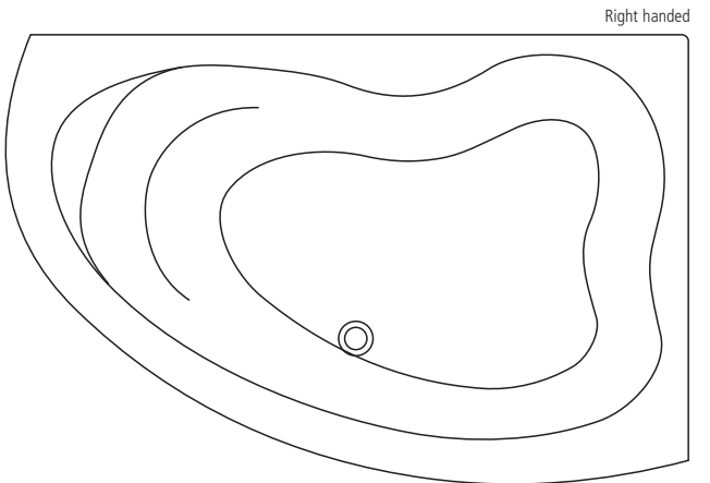
Create 160cm Idealform offset corner bath right handed 1600 x 1050mm height – floor to rim 550mm bath screen/over-bath enclosure height – 1500mm
