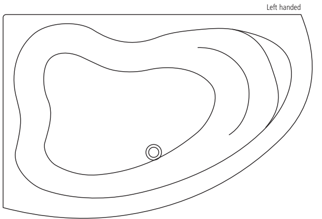
Create 160cm Idealform offset corner bath left handed 1600 x 1050mm height – floor to rim 550mm bath screen/over-bath enclosure height – 1500mm
