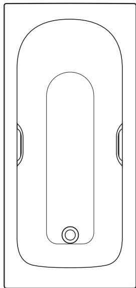
Harrow 150 150 x 70cm Idealform or Idealform Plus+ bath with optional grips, 1500 x 700mm height – floor to rim 540-560
