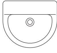
Edge 56cm semi-countertop basin w560 x d450mm
