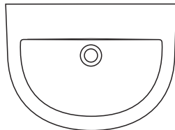
Washpoint 65cm basin w650 x d480mm
