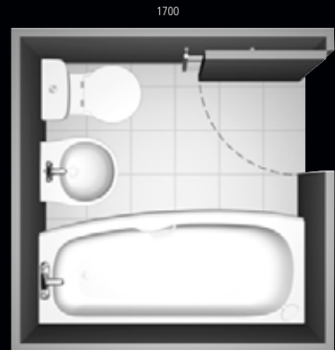
Space 44cm narrow basin and close coupled wc suite Studio 170cm Idealform spacemaker bath (right handed)
