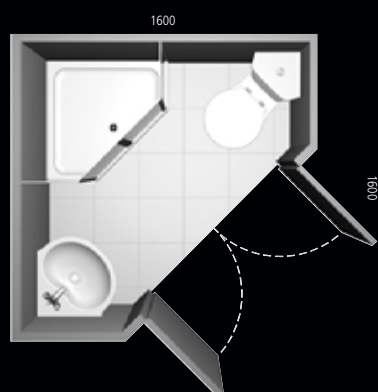
Space 56cm corner basin, corner close coupled wc suite and corner shower tray Joy in-fold shower enclosure Call 0800 590311 for an Ideal Standard Showers Studio Collection brochure
