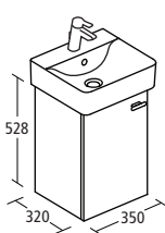
E6442-- 350mm Cube basin unit* For 40cm Cube basin 1 door
