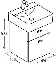
E6444-- 450mm Cube basin unit* For 50cm Cube basin 2 drawers
