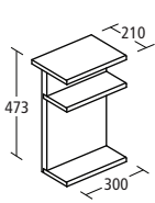
E6466-- Sphere/Arc shelf link unit Links Sphere/Arc basin unit with other freestyle or fitted units. Available in 3 colour options
