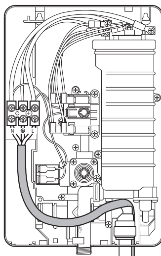
Bottom right * cable entry
