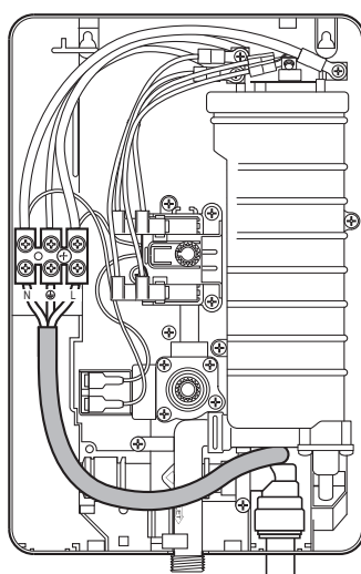
Rear bottom right cable entry
