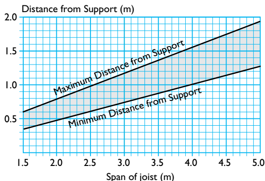
Fig. 31 Graph showing dimension of joist drilling zone from support
