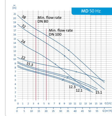
MULTILIFT MD
