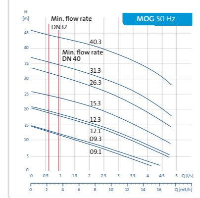
MULTILIFT MOG
