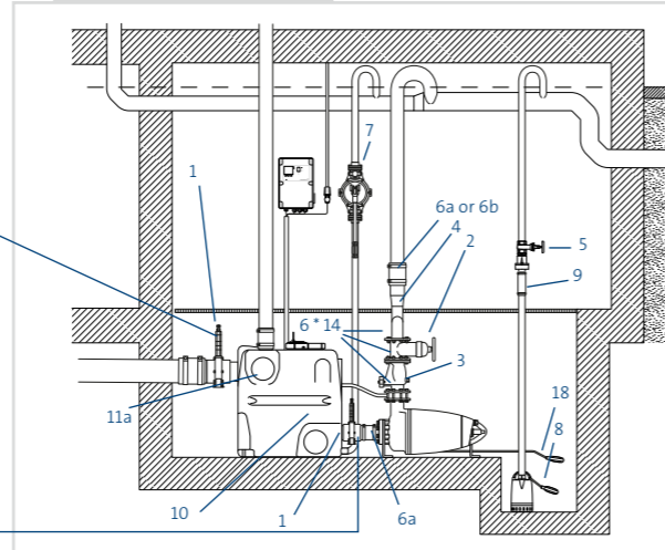
MULTILIFT MD1/MDV
