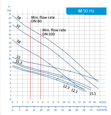
MULTILIFT M
