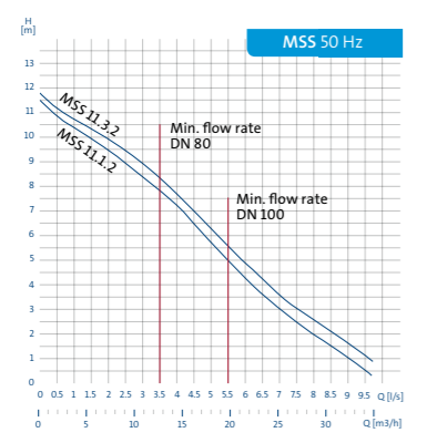
MULTILIFT MSS
