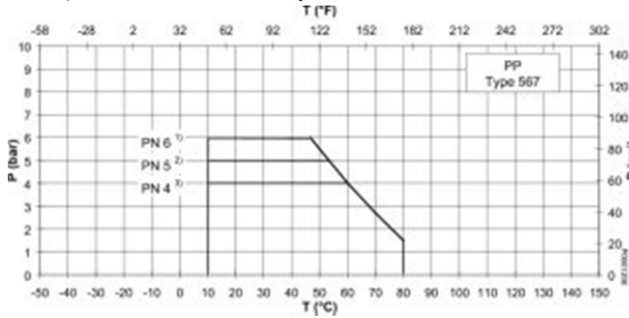
P: Permissible pressure in bar, psi; T: Temperature in °C, °F 1) DN350 - 400; 2) DN450; 3) DN500 – DN 600
