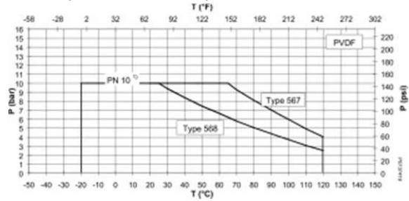
P: Permissible pressure in bar, psi; T: Temperature in °C, °F 1) DN50 - DN300
