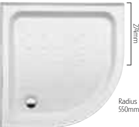
Quadrant 800mm Internal: 800 x 800mm External: 824 x 824mm White D85330
