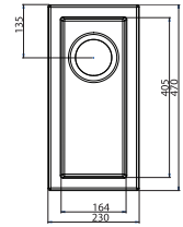
CUT OUT – 206 x 446mm U/M CUTOUT – 159 x 399mm, corner radiuses 6mm
