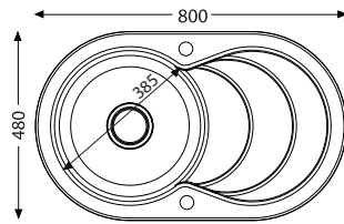
CUTOUT 776 x 456mm Corner radiuses 228mm
