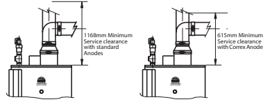
LCSC39 and LCSC59 Alternative Flue Systems
