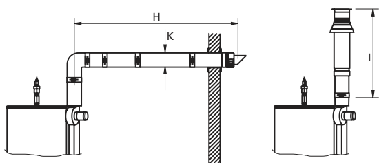
CSC78 and CSC93 Alternative Flue Systems
