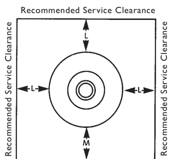
Plan View
