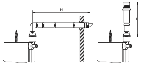
CSC39 and CSC59 Alternative Flue Systems
