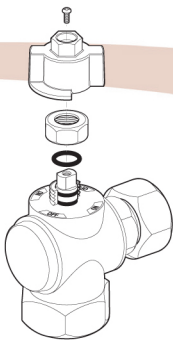
Bleed valve
