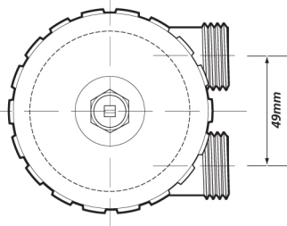
See how the MagnaClean Professional's 360° valves provide multiple installation options
