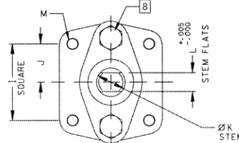
ACTUATOR MOUNTING
