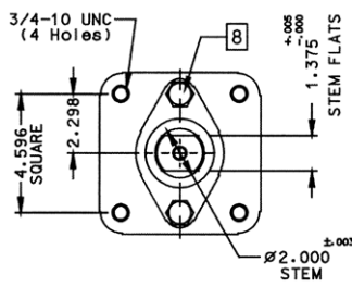
ACTUATOR MOUNTING: 8"
