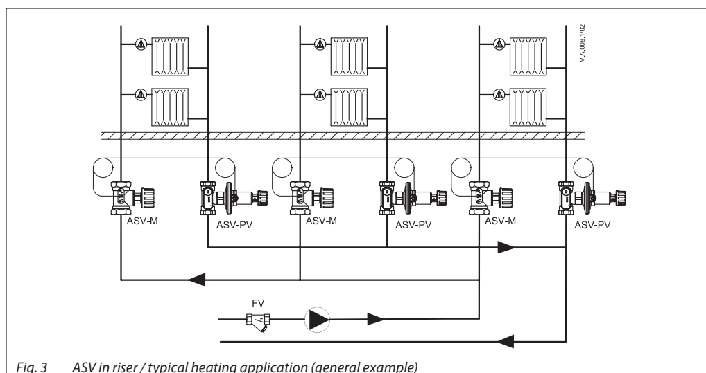
Fig. 3 ASV in riser / typical heating application (general example)
