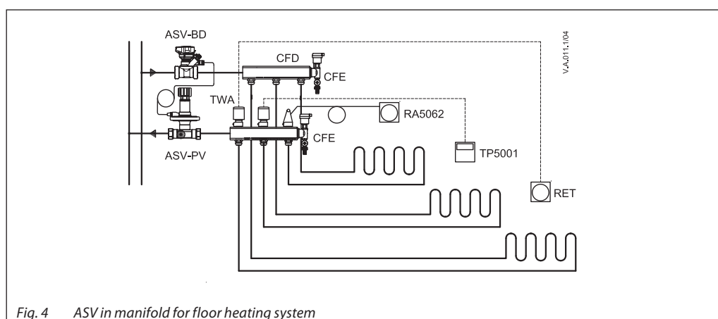
Fig. 4 ASV in manifold for floor heating system
